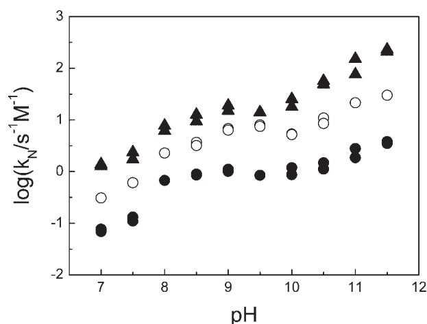
Figure 4. Plots of \log k_N versus pH for the reactions of TNPC (▲), DNPC (○) and NPC (●) with PL, in aqueous solution, at 25°C and ionic strength 0.1 M (KCl)
